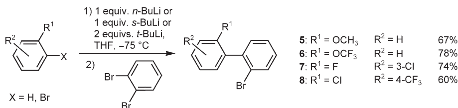
Scheme 3. Synthesis of ortho,ortho' -disubstituted biaryls by homo - and hetero -aryl/aryl coupling.
