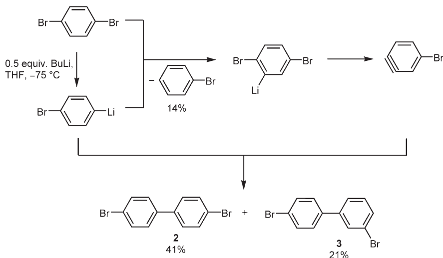
Scheme 2. Experimental evidence for an aryne intermediate.
