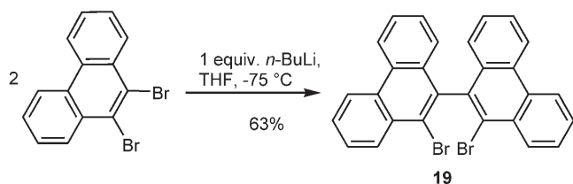
Scheme 5. Synthesis of an ortho,ortho' -tetrasubstituted biaryl by homo -aryl/aryl coupling.
