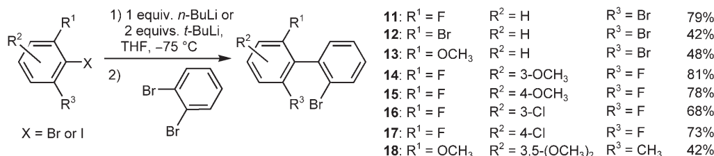
Scheme 4. Synthesis of ortho,ortho' -trisubstituted biaryls by homo - and hetero -aryl/aryl coupling.
