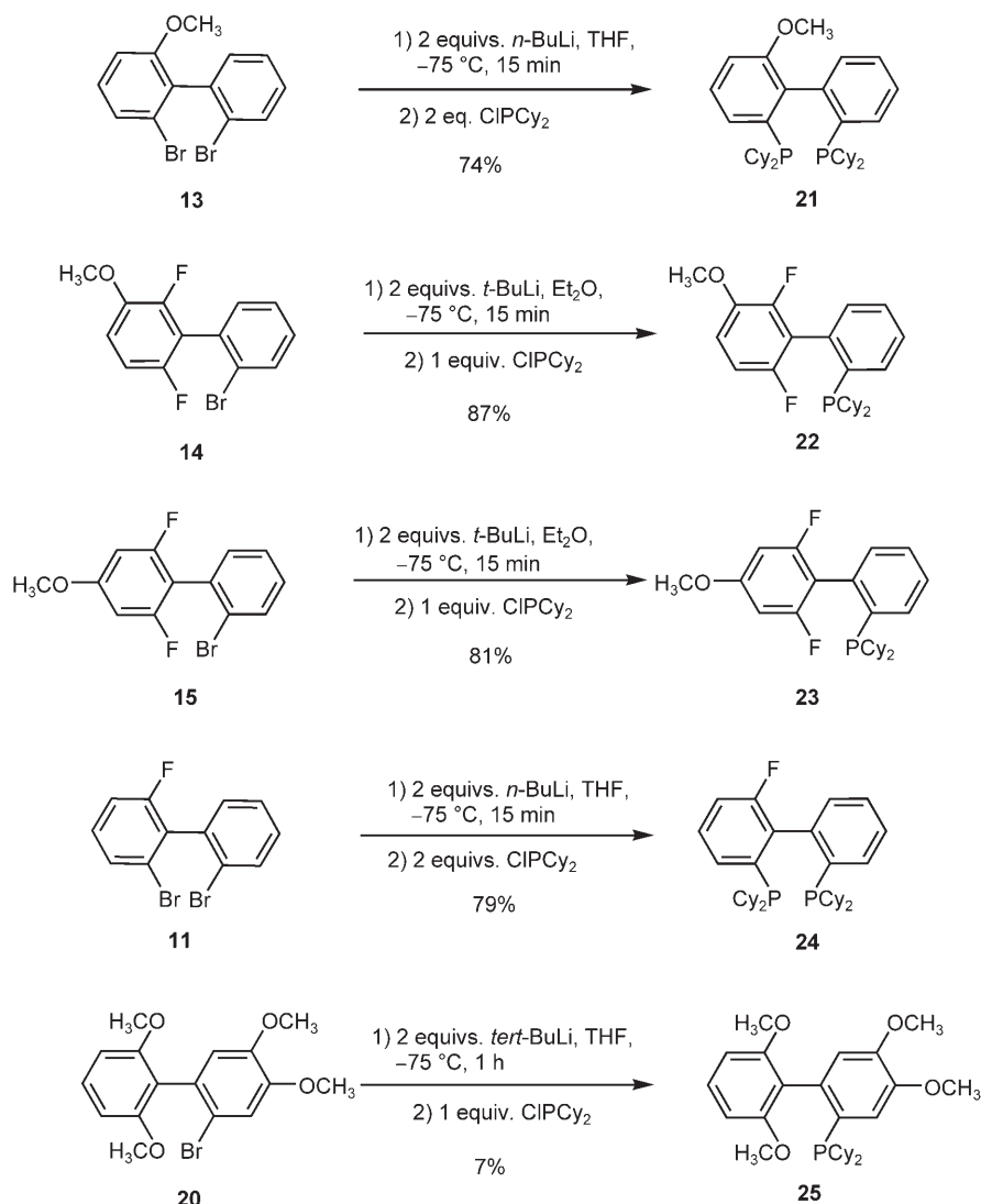
Scheme 7. Synthesis of C 1 -symmetric biarylmono- and diphosphines.
