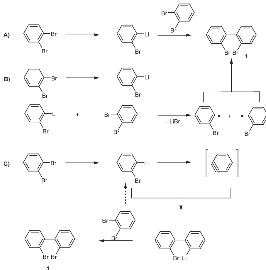
Scheme 1. Possible pathways for the butyllithium promoted formation of 2,2'-dibromobiphenyl ( 1 ).
