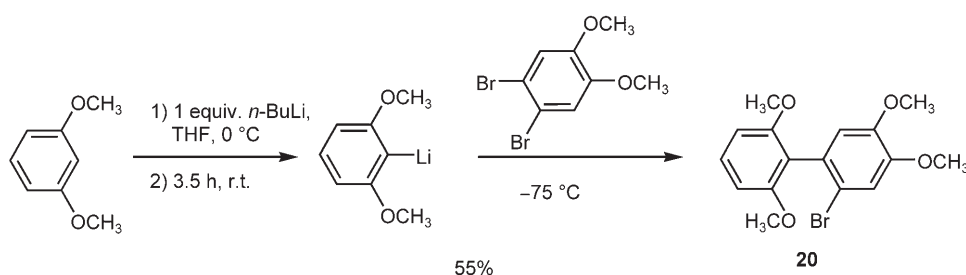
Scheme 6. Aryne coupling using 1,2-dibromoveratrole as aryne source.
